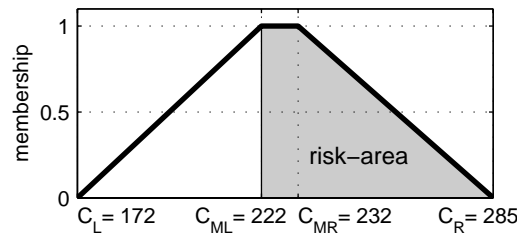
Figure 24: Risk assessment of range of costs.
