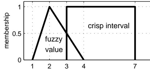
Figure 8: Fuzzy element of a crisp interval.
