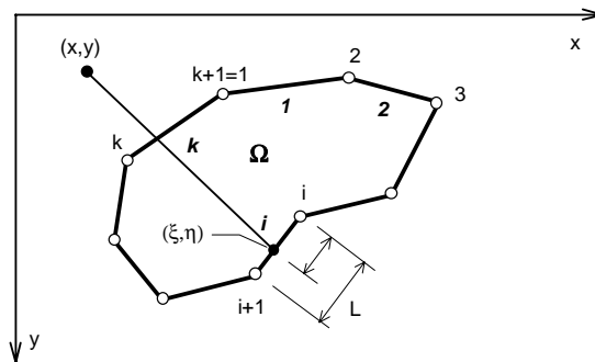
Figure 3: Polygonal approximation of the loaded area.
