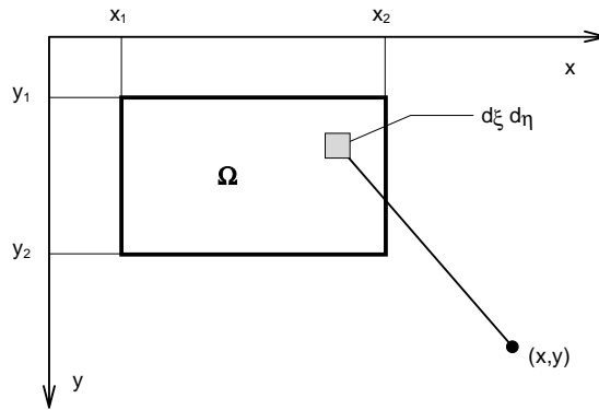
Figure 4: Uniformly distributed load over a rectangular area.
