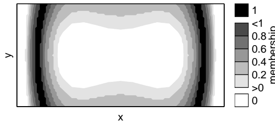
Figure 9: \tilde{M}_x \in [7.5, 10] kNm/m.
