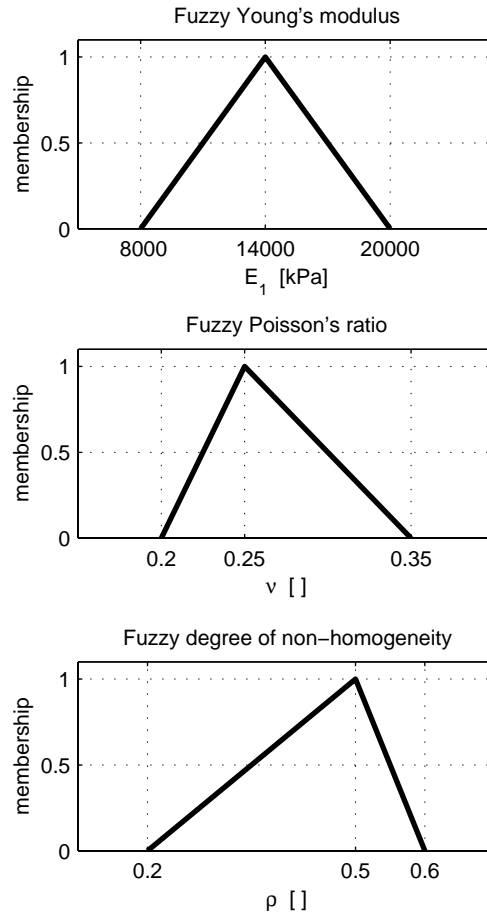
Figure 5: Membership functions of \tilde{E}_1 , \tilde{\nu} and \tilde{\rho} .
