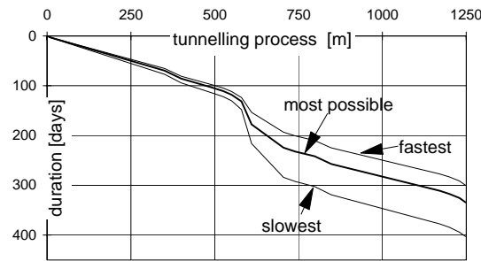
Figure 18: Time/velocity diagram.
