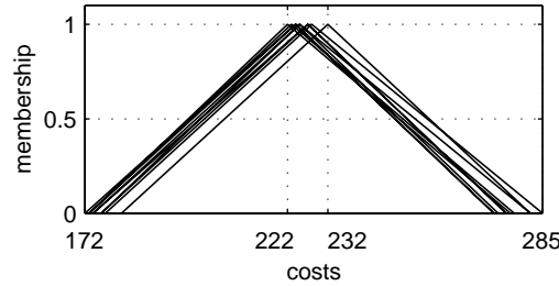
Figure 23: Fuzzy cost variations at duration T = 29 .
