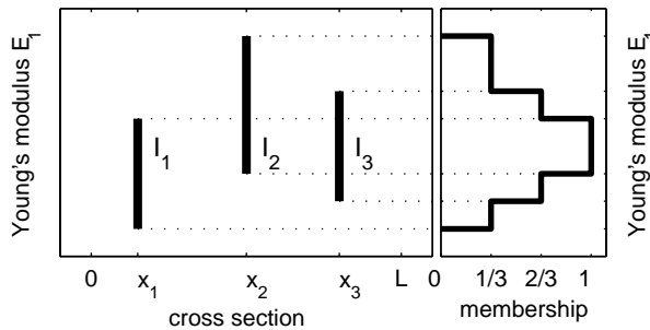
Figure 11: Determination of fuzzy number \tilde{E}_1 .
