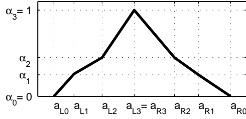
Figure 2: Polygonal fuzzy number.
