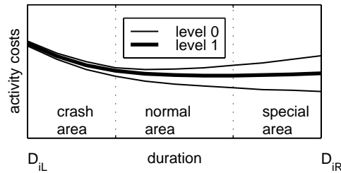
Figure 21: Fuzzy time/cost dependence.
