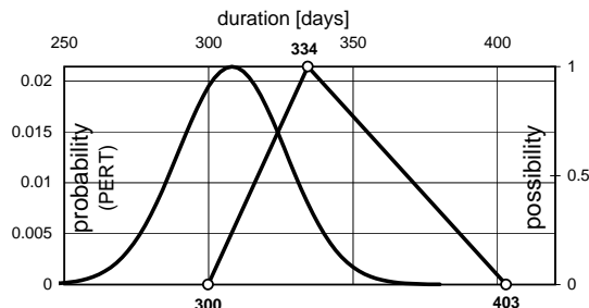
Figure 17: Probability/possibility distribution of total duration.
