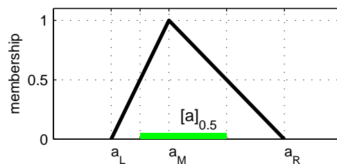
Figure 1: Triangular fuzzy number.
