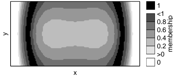
Figure 10: \tilde{M}_x \in [10, 12.5] kNm/m.
