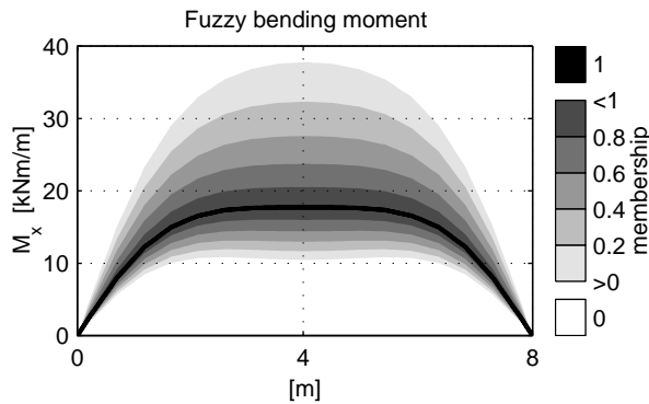
Figure 7: Fuzzy bending moment \tilde{M}_x along a section.
