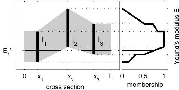
Figure 12: Determination of fuzzy number \tilde{E}_1 .
