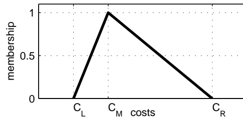
Figure 20: Membership function for cost of activity at fixed duration.
