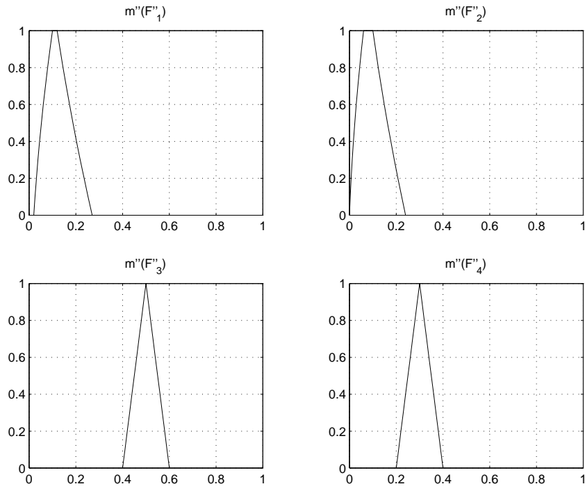
Figure 3: Result of the combination of two FBSs.
