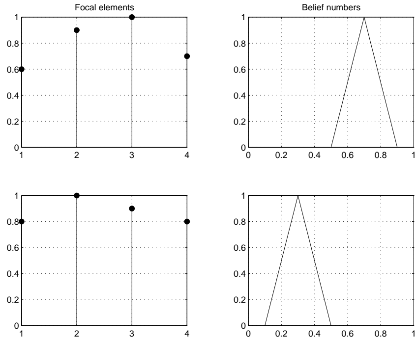
Figure 5: Yager normalization of the FBS shown in Figure 4. Left: normalized focal elements F_i^\circ . Right: fuzzy belief numbers \tilde{m}^\circ(F_i^\circ) after normalization.
