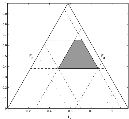
Figure 1: Representation of an IBS (gray region) in the probability simplex. Original inequality constraints and tightest bounds are represented as dotted and dashed lines, respectively
