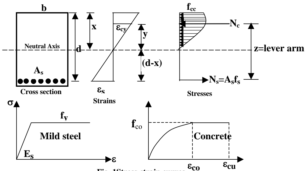
Fig. 1 Stress-strain curves
